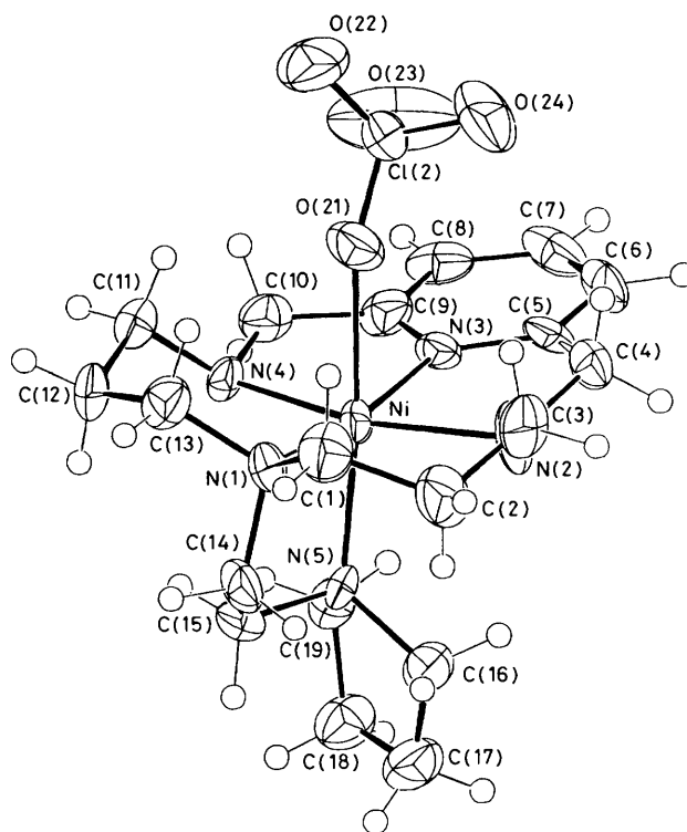
Figure 1. X-Ray structure of [Ni(L 1 )(OCIO 3 )] [ClO 4 ] showing the atomic numbering scheme
