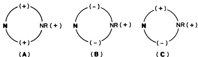
Figure 2. Schematic representation of the three possible isomers of square-planar [Ni(HL)] 3+ ions (L = L 1 or L 2 ); (+) and (-) represent the positions of either macrocyclic NH groups or N pendant arm (R), either above (+) or below (-) the macrocyclic ligand plane. The pyridine-N atom is in bold type. (C) is enantiomeric
